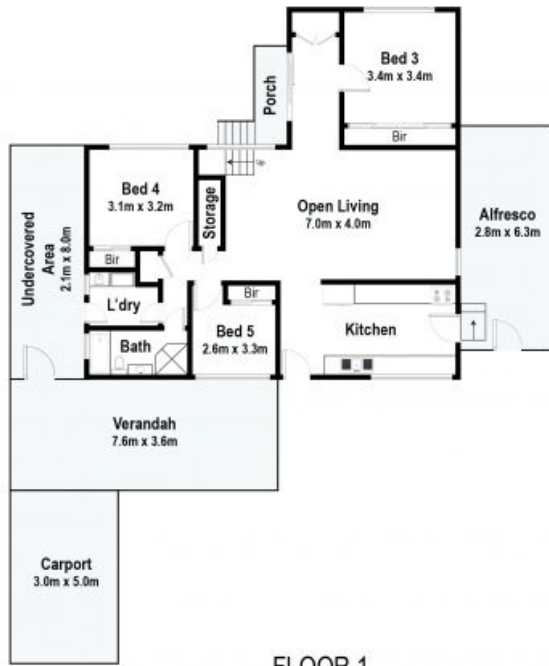
FLOOR 1
