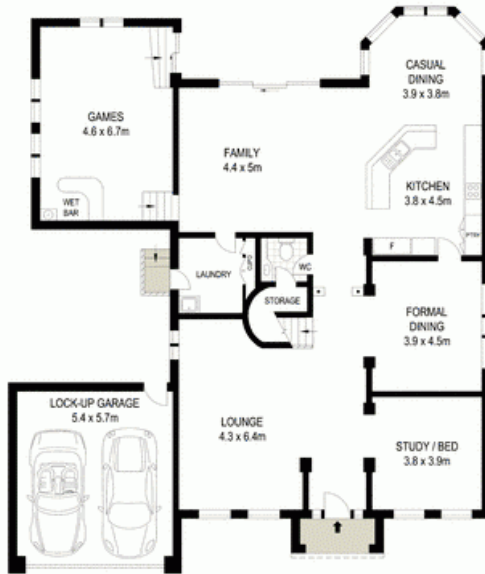
LOWER LEVEL
